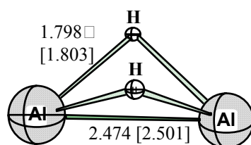
\angle Al-H-Al 86.9 [87.9] \angle H-Al-H 70.8 [71.4] Dih H-Al-Al-H 106.0 [108.3] 5 ( C_{2v} ) ( ^1A_1 ) nonplanar dibridged
