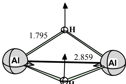
\angle Al-H-Al 105.6 \angle H-Al-H 71.5 Dih H-Al-Al-H 149.8 planar dibridged-nonplanar dibridged TS1-5 ( C_{2v} ) ( ^1A_1 ) 155 icm^{-1}
