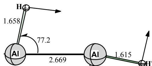
\angle Al-Al-H' 168.9 trans-monobridged TS3-4 ( C_s ) ( ^1A' ) 286 icm^{-1}
