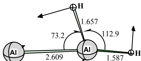
branched-monobridged TS2-4 ( C_s ) ( ^1A' ) 297 icm^{-1}
