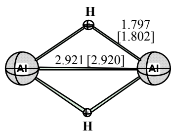
\angle Al-H-Al 108.7 [108.2] 1 ( D_{2h} ) ( ^1A_g ) planar dibridged
