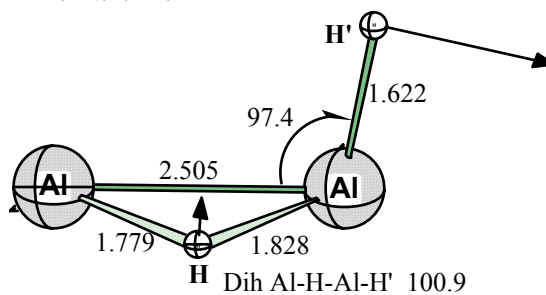
planar dibridged-monobridged TS1-4 ( C_1 ) ( ^1A ) 281 icm^{-1}
