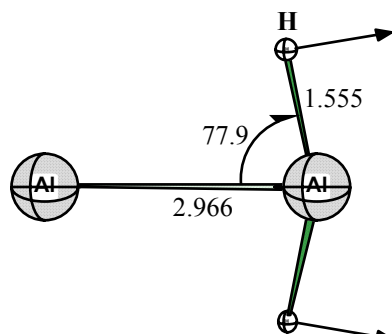
planar dibridged-bridged TS1-2 ( C_{2v} ) ( ^1A_1 ) 1032 icm^{-1}
