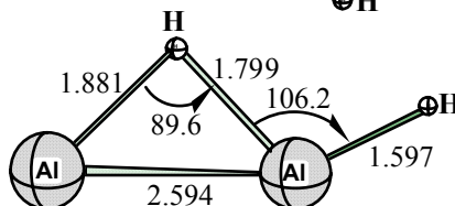
4 ( C_s ) ( ^1A' ) monobridged
